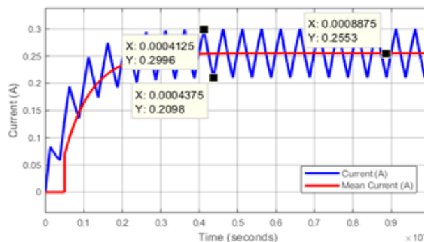
Figure (1.2): Current response (Blue) and the mean value of the current (Red)
