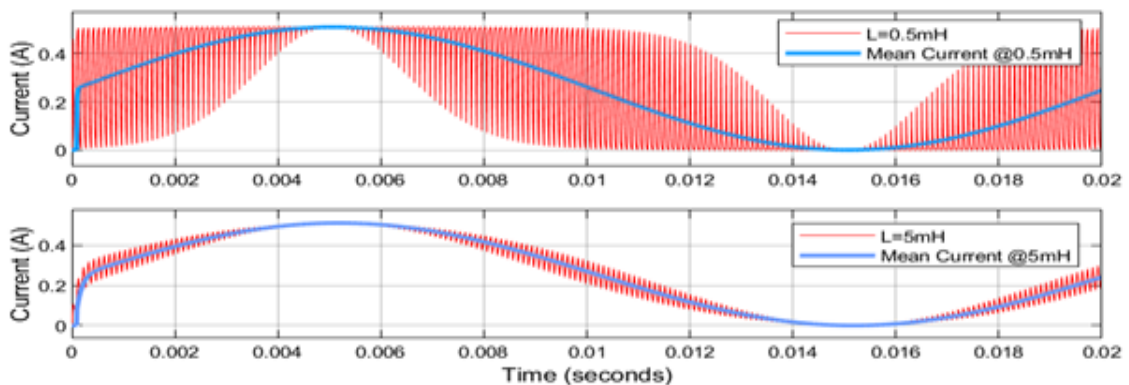
Figure (1.9): The effect of inductance load to output waveform voltage.
