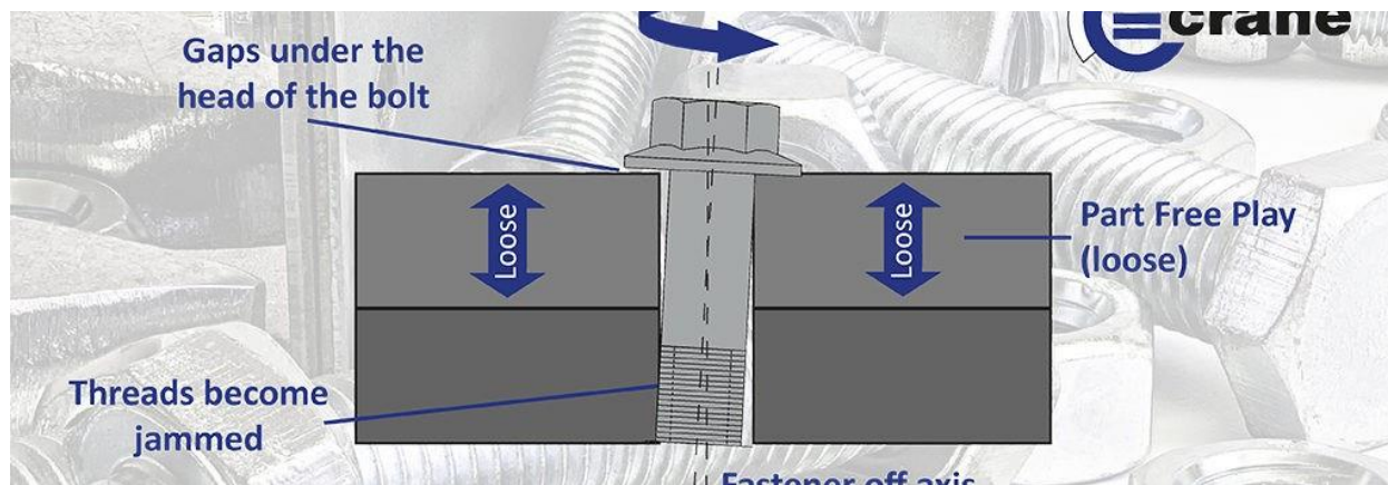
Figure 1. Cross-threading nut and bolt.
